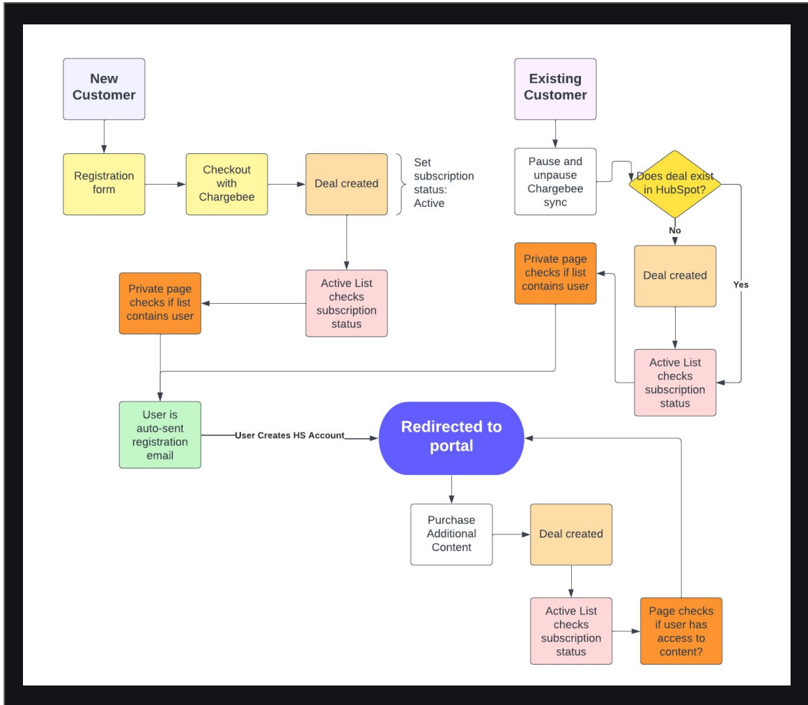
Lucidchart for mockup of a User Access Flow.
